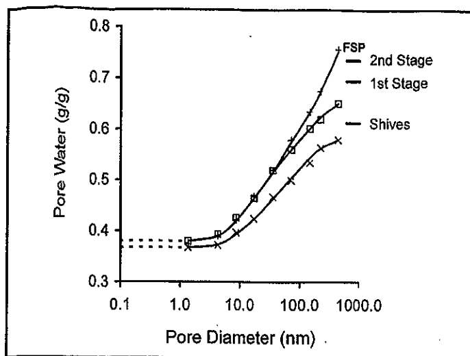
Fig. 7. Pore size distribution for spruce TMP: first-stage fibres (□); second-stage fibres (+); and first-stage shives (×).
