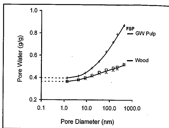
Fig. 8. Pore size distribution for spruce groundwood whole pulp (+) and spruce wood without boiling (×) and after boiling (□).
