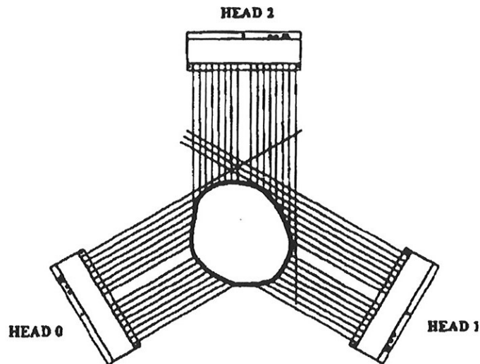
Figure 1. Schematic description of an optical 3D surface scanner (Dashner 1993).
