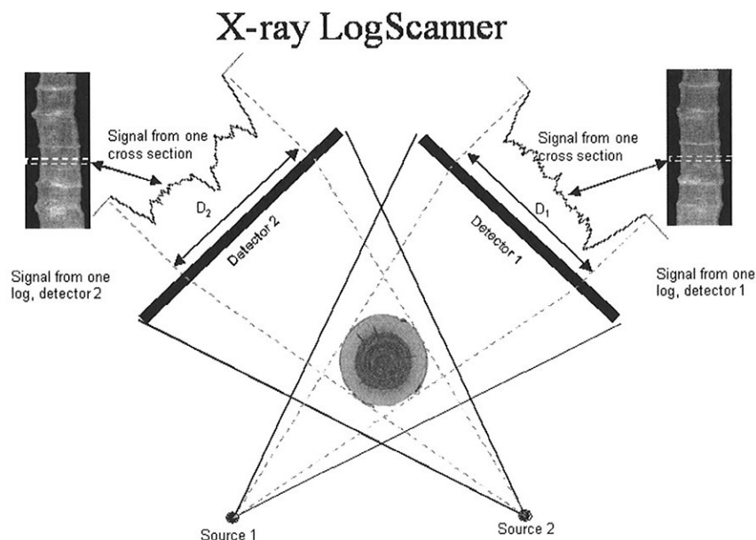
Figure 2. Schematic description of the X-ray LogScanner developed by Grundberg and Grönlund (1995), image from Oja et al. (1998).
