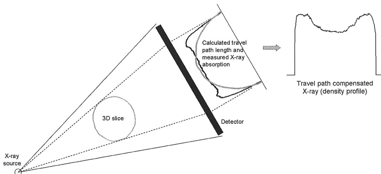
Figure 3. Principle for density profile calculation from an X-ray (black) cross-section and a 3D (gray) cross-section.
