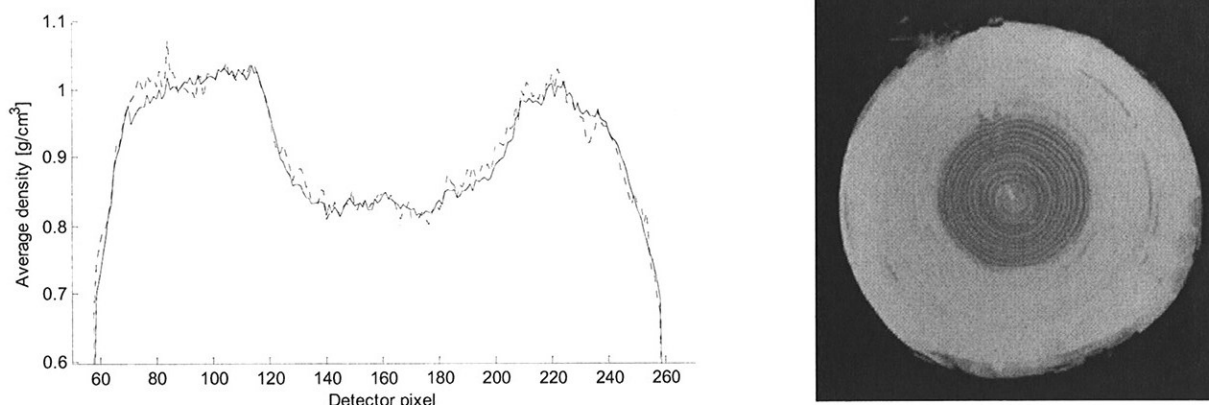
Figure 5. (a): Green density profile of a log cross-section, the dotted line shows a single cross-section and the solid line shows an average over five neighbouring cross-sections. (b): CT image showing the corresponding log cross-section. Dark pixels represent low density while bright pixels represent high density.
