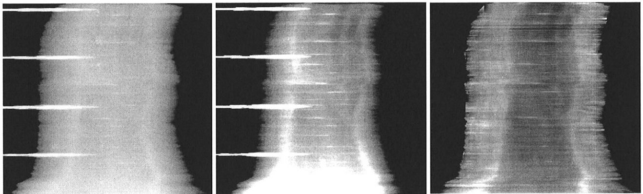
Figure 4. (a), (b): Raw LogScanner data, X-ray absorption depends on density as well as travel path. (a) shows the full data range whereas (b) shows a zoomed data range, better exposing internal artefacts as well as the varying absorption along the log due to varying diameter. (c): Travel path compensated LogScanner data showing the density profile of the log. Uncertainty in the combination of 3D and X-ray data can be seen as bright or dark radial lines at the edge of the log, where the relative uncertainty of the travel path is greatest.
