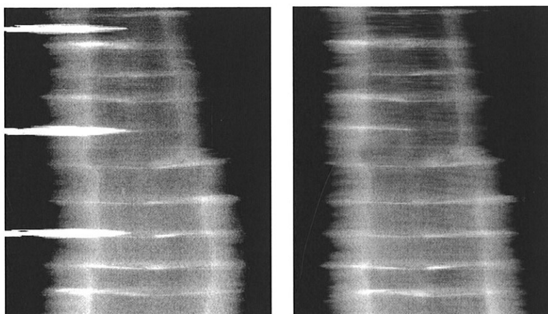
Figure 6. LogScanner data from an industrial installation (left). LogScanner data simulated from CT images (right).
